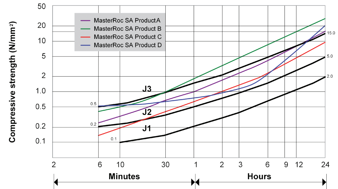
Compressive strength of sprayed concrete
